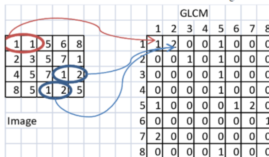
Figure 4. GLCM calculation
