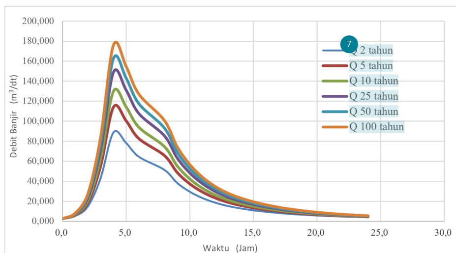
Gambar 1. Hidrograf debit banjir das oba metode nakayasu
