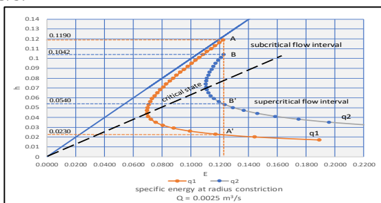
Fig. 13: Specific energy at radius constriction with Q = 0.0025 \text{ m}^3/\text{s}
