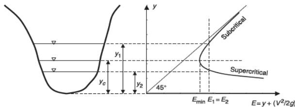
Fig. 5: Specific energy diagram [9]
