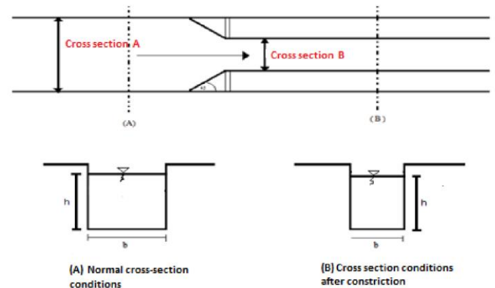
Fig. 3: Cross-section on Transitional type refinement. [4]
