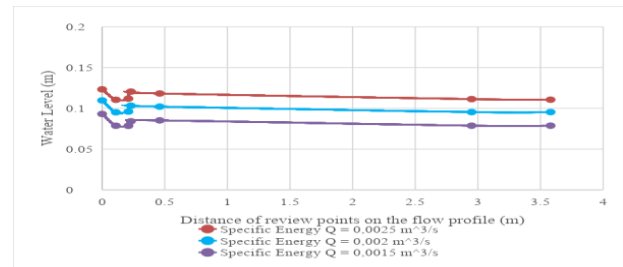
Fig. 9: Specific Energy and water level with a transition with a discharge of 0.0025 m 3 /s, 0.0020 m 3 /s, and 0.0015 m 3 /s.
