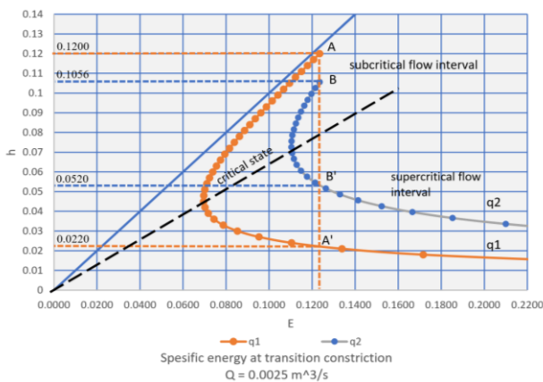
Fig. 12: Specific energy at transition constriction with Q = 0.0025 \text{ m}^3/\text{s}
