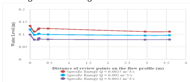
Fig. 8: Specific Energy and water level with a sudden constriction with a discharge of 0.0025 m 3 /s, 0.0020 m 3 /s, and 0.0015 m 3 /s.
