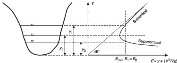
Fig. 5: Specific energy diagram [9]
