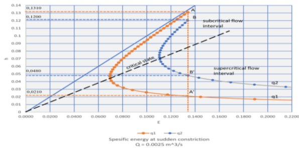
Fig. 11: Specific energy at sudden constriction with Q = 0.0025 \text{ m}^3/\text{s}
