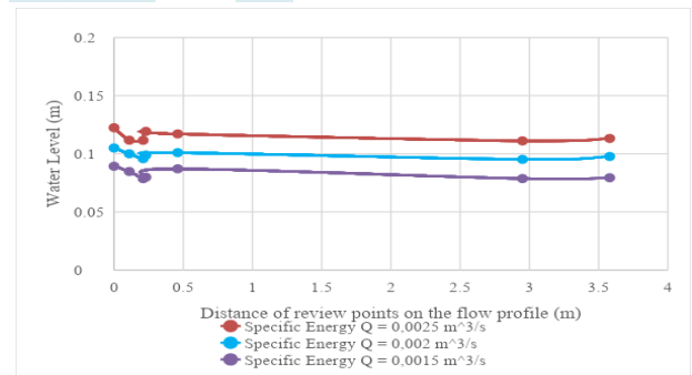
Fig. 10: Specific Energy and water level with a radius type with a discharge of 0.0025 m 3 /s, 0.0020 m 3 /s, and 0.0015 m 3 /s.
