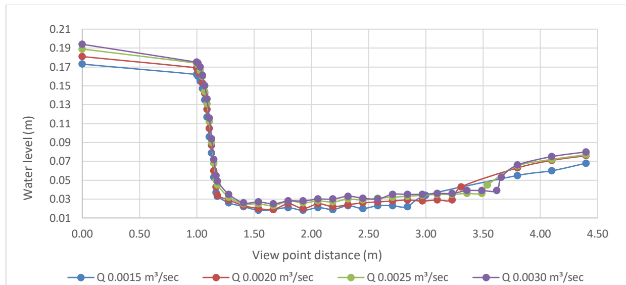
Fig 8:- Graph of the relationship between the height of the water level dihu with the review distance at a height of 0.120 m against the variation of discharge.
