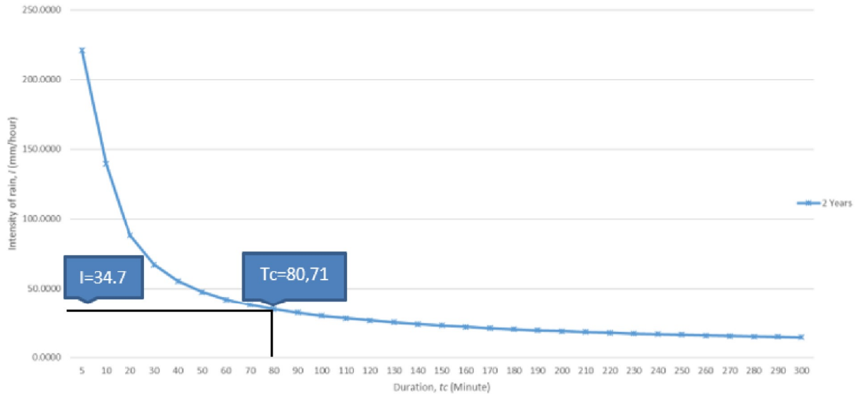
Fig 3:- Graph of rainfall determination based on tc value
