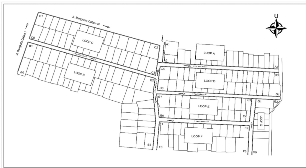
Fig 4:- Drainage network map
