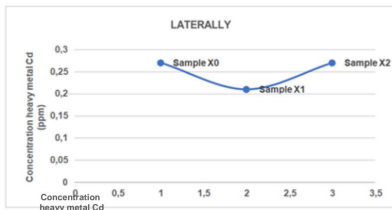
Figure 6. Laterally cadmium concentration in the samples of X0, X1, and X2, with each distance of 5 m (0, 5, and 10 m) from the garbage pile at the sampling area.
