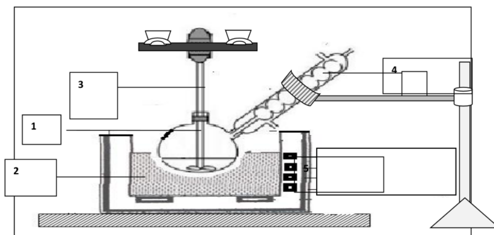
Figure.1 The experiment setup for transesterification process assisted by ultrasonic, 1. Batch reactor, 2. ultrasonic, 3. stirring bar 4. reflux condenser, 5. power control instrument, time setting.
